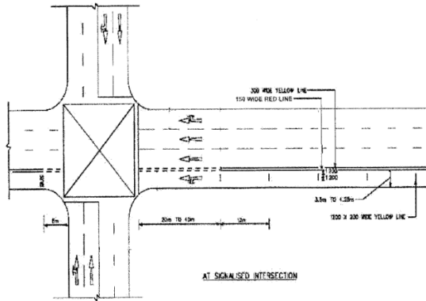
AT SIGNALISED INTERSECTION FOR FULL-DAY BUS LANE
