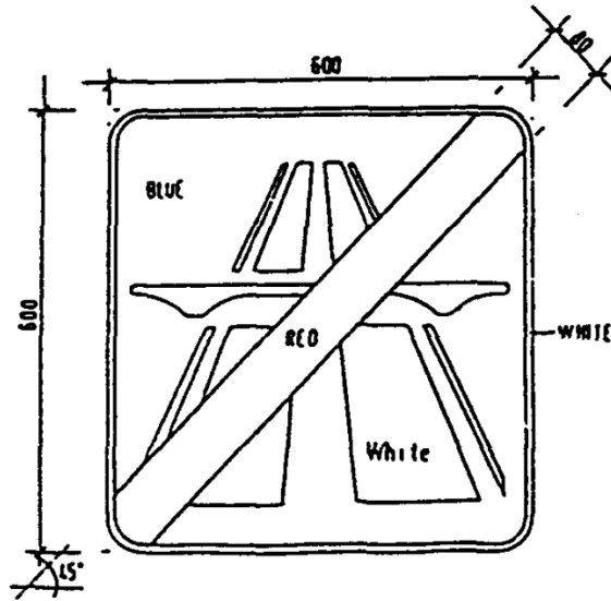
END OF EXPRESSWAY
