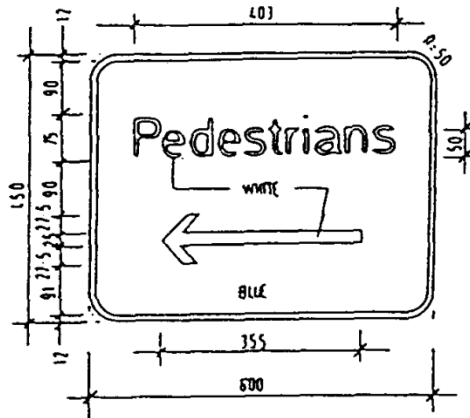
DIRECTION OF TEMPORARY PEDESTRIAN ROUTE
