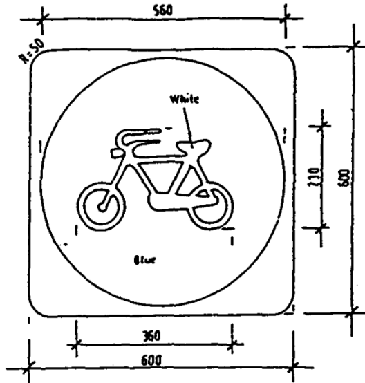
COMPULSORY CYCLE TRACK
