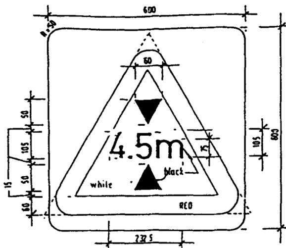
HEIGHT LIMIT AHEAD
