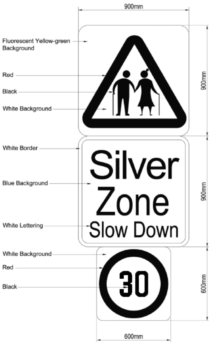
SILVER ZONE, 30 KM/H
