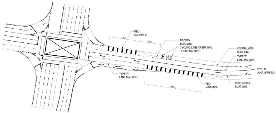
A part-day bicycle lane at a signalised intersection.
