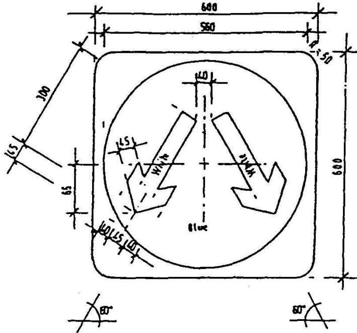
PASS EITHER SIDE
