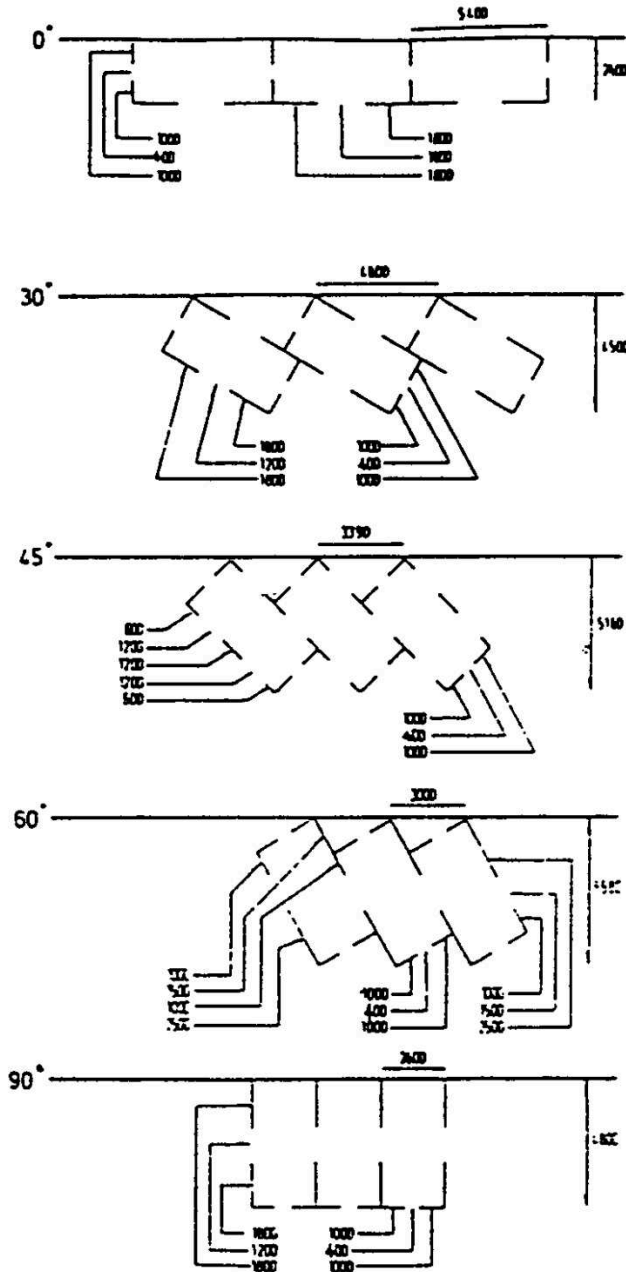
TYPICAL ARRANGEMENT OF PARKING LOTS
