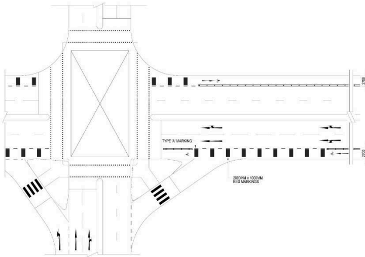
A full-day bicycle lane at a signalised intersection.
