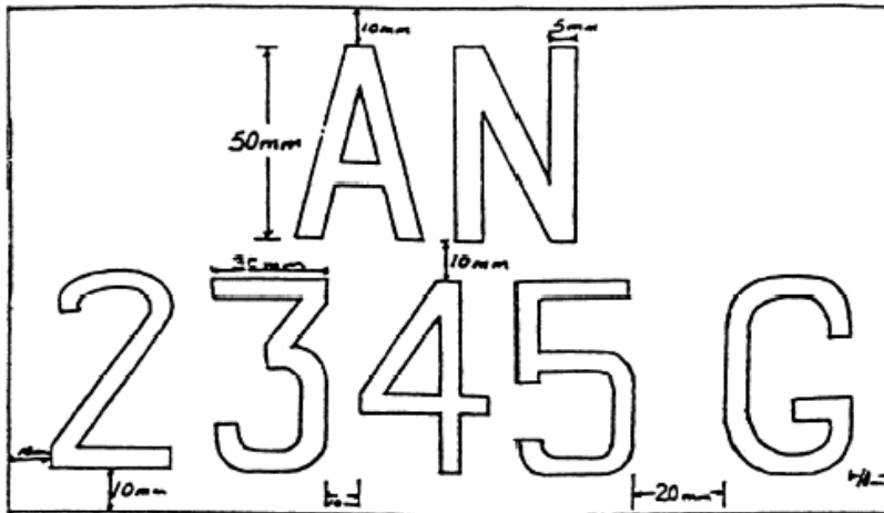
Dimensions are all in mm.
