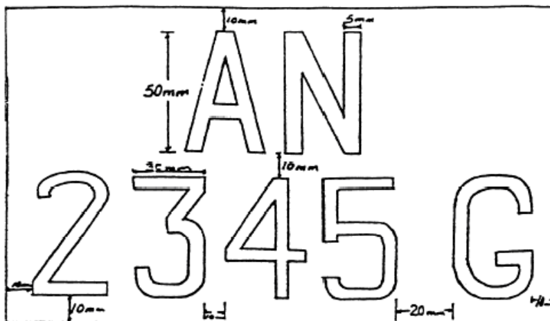
Dimensions are all in mm.
