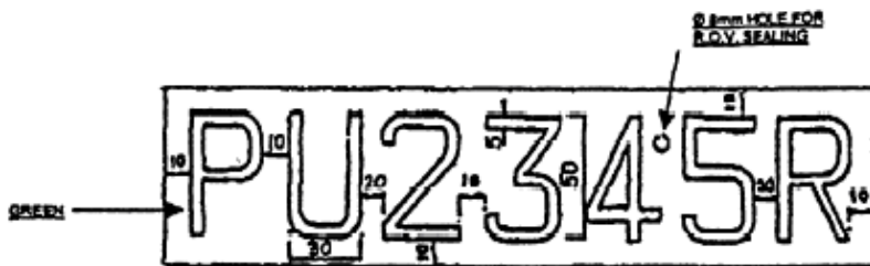
Dimensions are all in mm.
