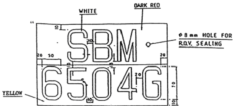
Dimensions are all in mm.
