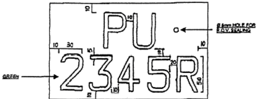
Dimensions are all in mm.
