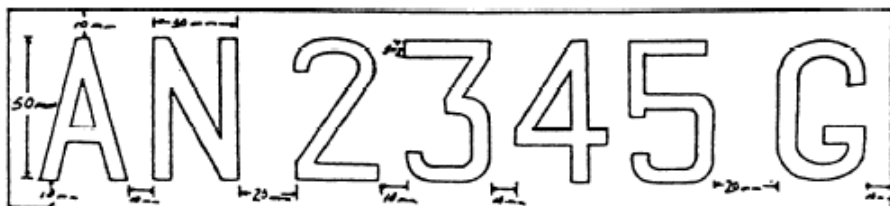
Dimensions are all in mm.
